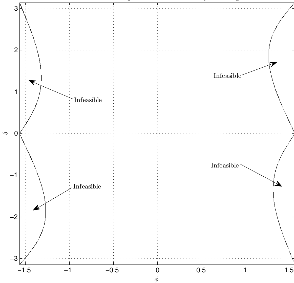
Feasible lean and steer angles for the benchmark bicycle above ground
